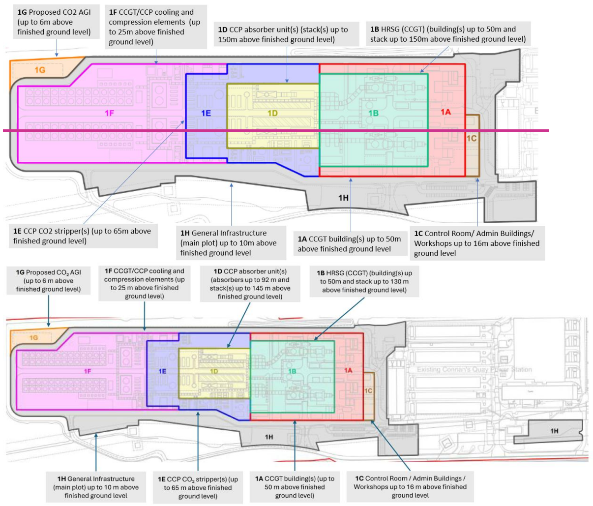
Plate 4-5: Details of Maximum Parameters Based on Tallest Components and Indicative Site Layout
